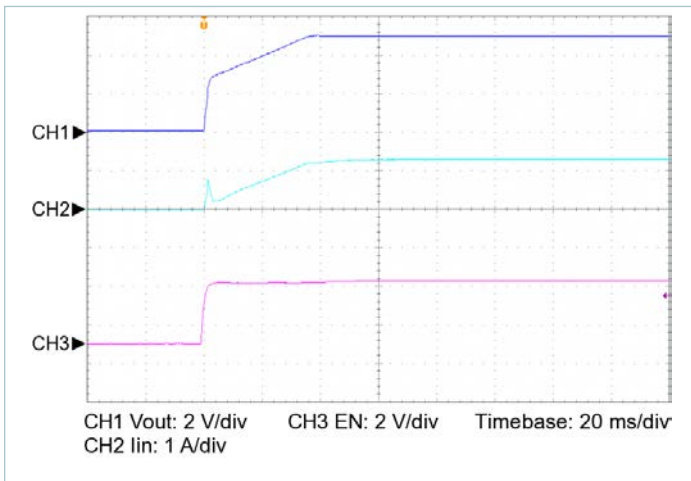
Figure 20 — Start up from EN, V_{IN} = 100\text{V} , C_{OUT\_EXT} = 20000\mu\text{F} , R_{LOAD} = 0.208\Omega
