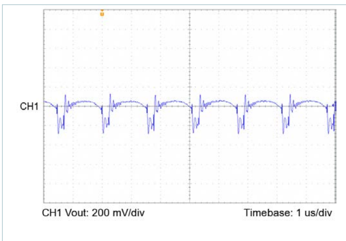
Figure 22 — Output voltage ripple, V_{IN} = 100\text{V} , V_{OUT} = 5.0\text{V} , C_{OUT\_EXT} = 1000\mu\text{F} , R_{LOAD} = 0.208\Omega
