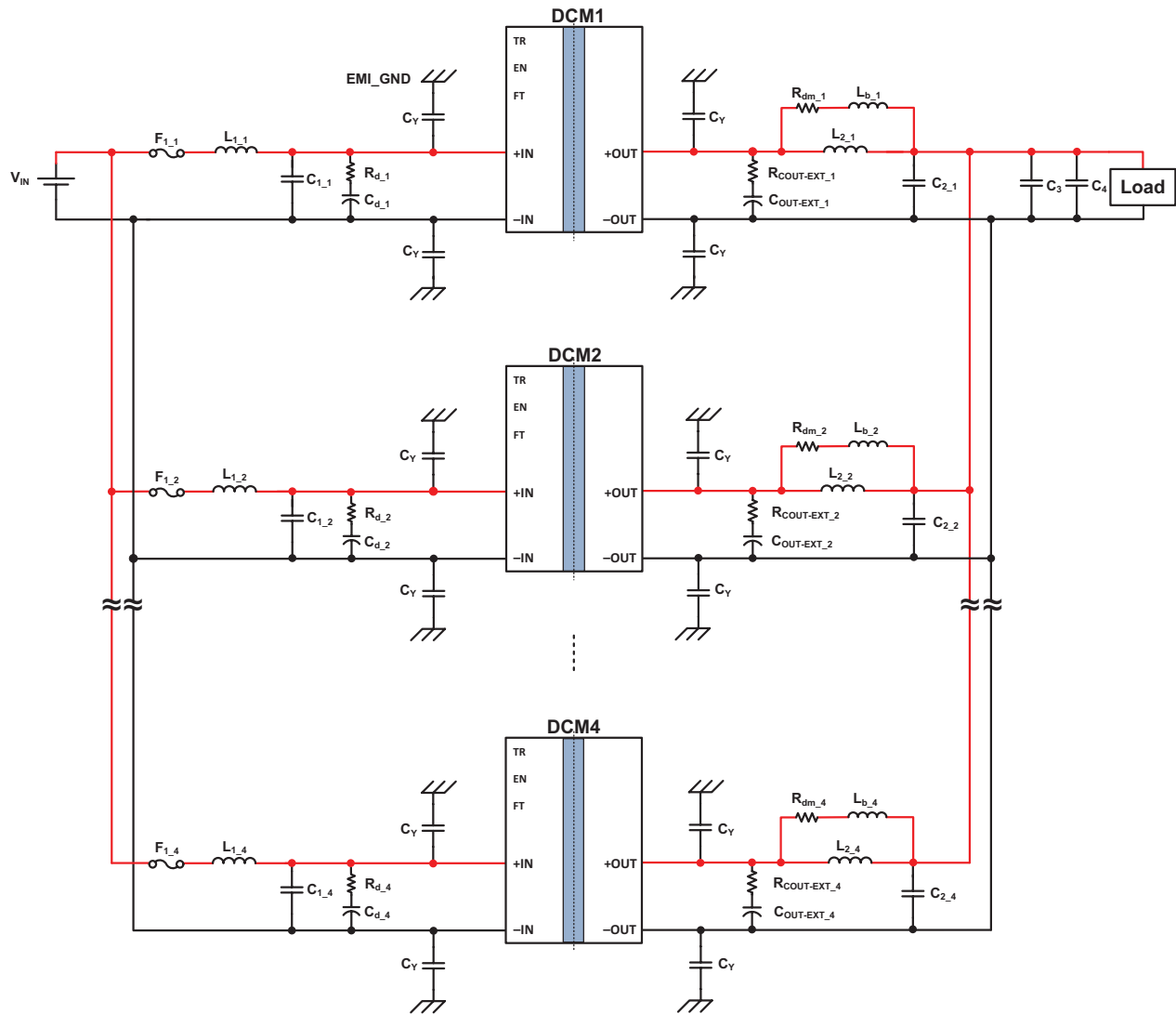
Typical application 1: DCM3623x50T26A6yzz in an array of four units
