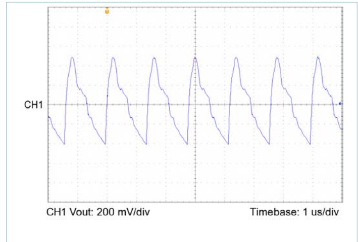
Figure 18 — Output voltage ripple, V_{IN} = 28\text{V} , V_{OUT} = 48.0\text{V} , C_{OUT\_EXT} = 200\mu\text{F} , R_{LOAD} = 7.200\Omega
