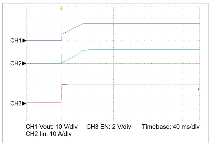
Figure 14 — Startup from EN, V_{IN} = 28\text{ V} , C_{OUT\_EXT} = 6800\text{ }\mu\text{F} , R_{LOAD} = 0.701\text{ }\Omega
