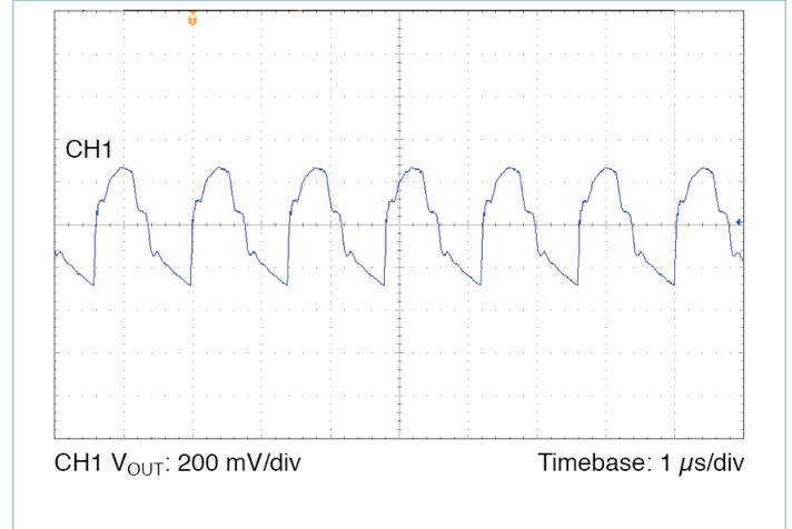
Figure 16 — Output voltage ripple, V_{IN} = 28\text{ V} , V_{OUT} = 15.0\text{ V} , C_{OUT\_EXT} = 680\text{ }\mu\text{F} , R_{LOAD} = 0.701\text{ }\Omega
