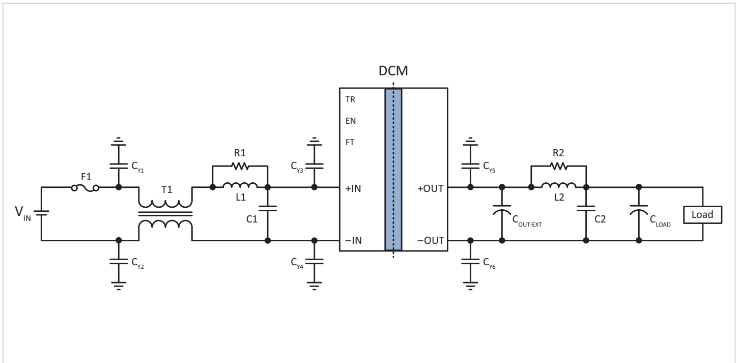
Typical Application 2: Single DCM3623x50M17C2y7z with common- and differential-mode input filters
