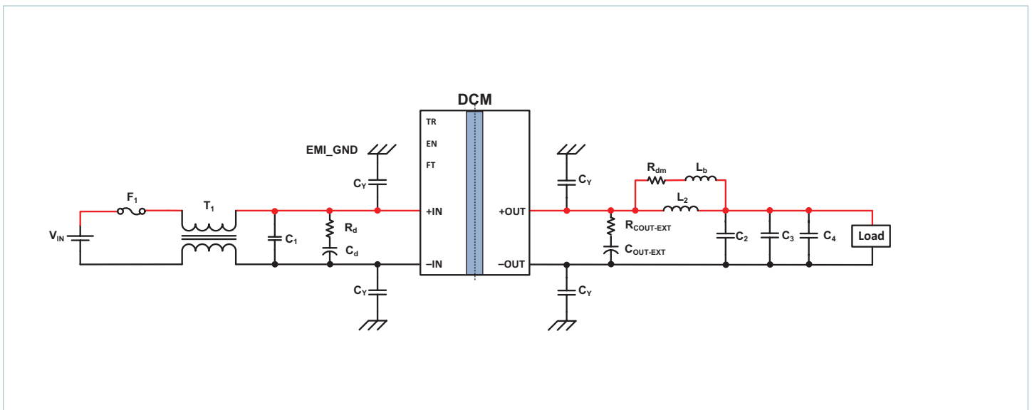
Typical application 2: single DCM3623x50M13C2y7z with common- and differential-mode input filters
