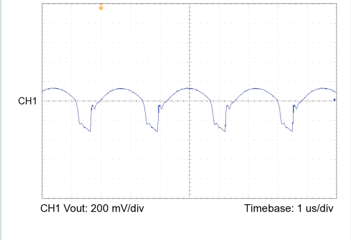
Figure 16 — Output voltage ripple, V_{IN} = 28\text{ V} , V_{OUT} = 3.3\text{ V} , C_{OUT\_EXT} = 1000\text{ }\mu\text{F} , R_{LOAD} = 0.091\text{ }\Omega
