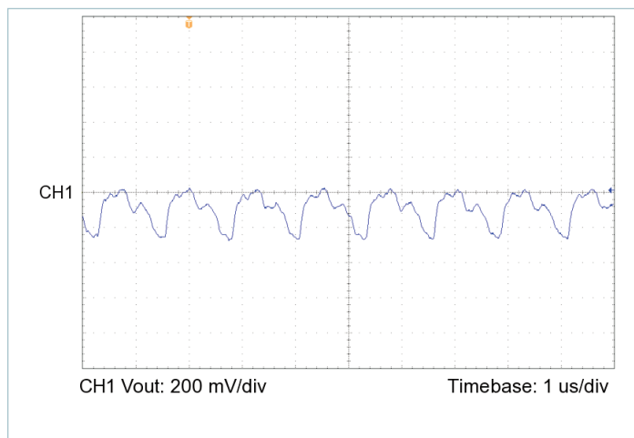
Figure 15 — Output voltage ripple, V_{IN} = 43\text{ V} , V_{OUT} = 12.0\text{ V} , C_{OUT\_EXT} = 1000\text{ }\mu\text{F} , R_{LOAD} = 1.429\text{ }\Omega
