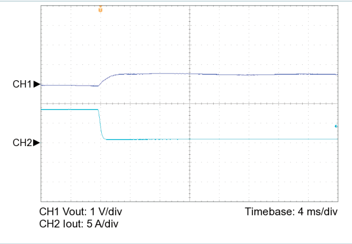
Figure 19 — 100% to 10% load transient response, V_{IN} = 43\text{ V} , nominal trim, C_{OUT\_EXT} = 1000\text{ }\mu\text{F}
