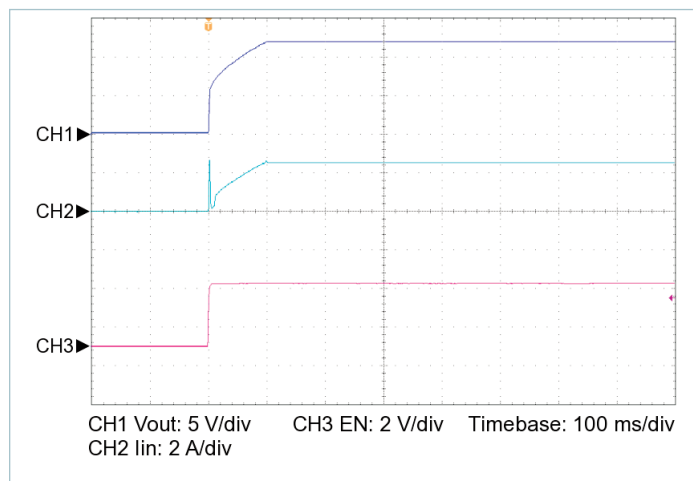
Figure 16 — Startup from EN, V_{IN} = 43\text{ V} , C_{OUT\_EXT} = 10000\text{ }\mu\text{F} , R_{LOAD} = 1.429\text{ }\Omega
