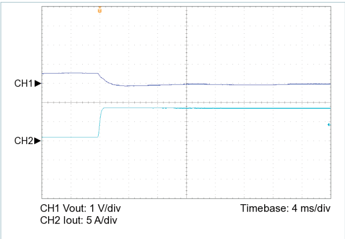
Figure 20 — 10% to 100% load transient response, V_{IN} = 43\text{ V} , nominal trim, C_{OUT\_EXT} = 1000\text{ }\mu\text{F}
