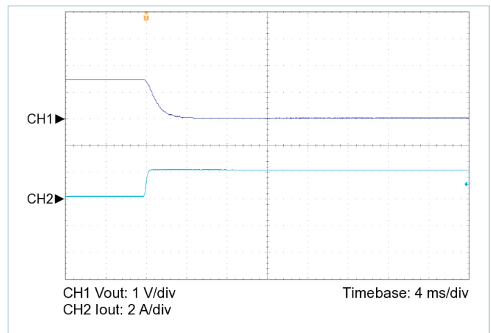
Figure 20 — 10% to 100% load transient response, V_{IN} = 30\text{ V} , nominal trim, C_{OUT\_EXT} = 220\text{ }\mu\text{F}
