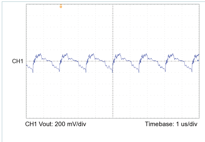
Figure 15 — Output voltage ripple, V_{IN} = 30\text{ V} , V_{OUT} = 28.0\text{ V} , C_{OUT\_EXT} = 220\text{ }\mu\text{F} , R_{LOAD} = 12.727\text{ }\Omega
