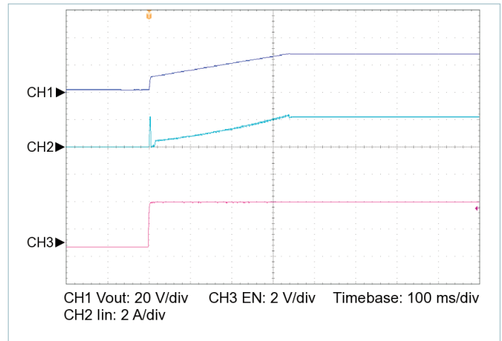
Figure 16 — Startup from EN, V_{IN} = 30\text{ V} , C_{OUT\_EXT} = 2200\text{ }\mu\text{F} , R_{LOAD} = 12.727\text{ }\Omega
