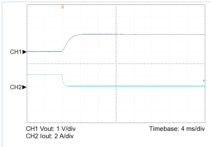
Figure 19 — 100% to 10% load transient response, V_{IN} = 30\text{ V} , nominal trim, C_{OUT\_EXT} = 220\text{ }\mu\text{F}
