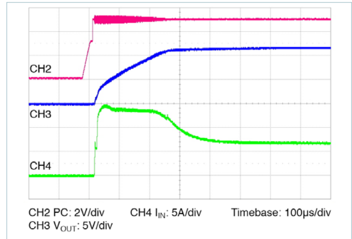
Figure 13 — Start up from application of PC; V_{IN} pre-applied C_{OUT} = 1000\mu\text{F}
