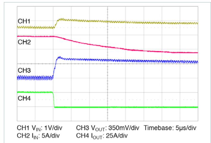
Figure 15 — 25 – 0A transient response: C_{IN} = 330\mu\text{F} , I_{IN} measured prior to C_{IN} , no external C_{OUT}
