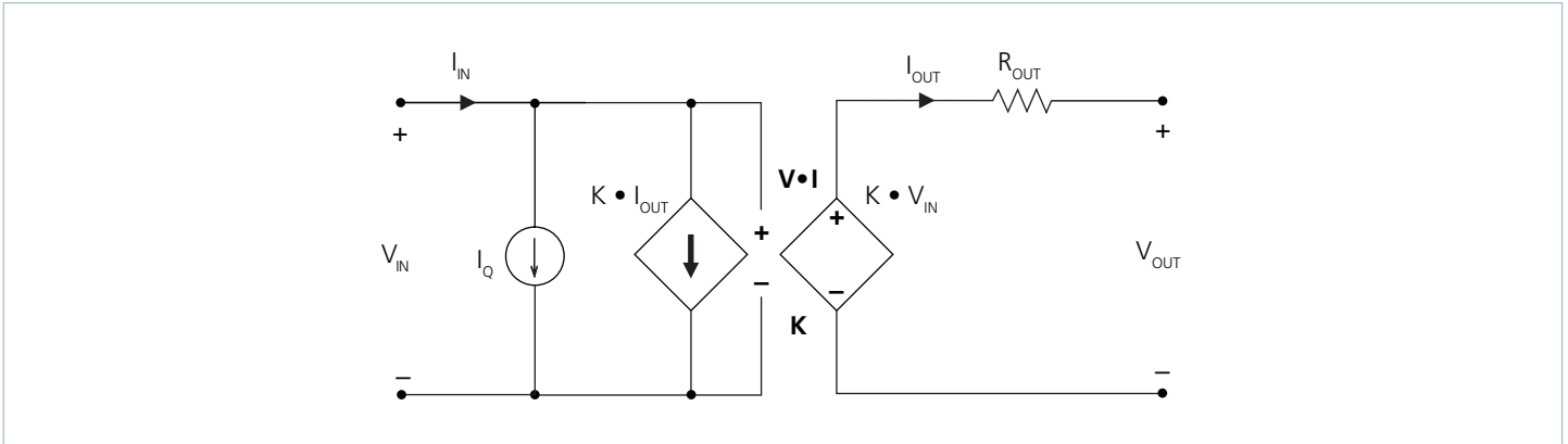
Figure 18 — VI Chip® module DC model
