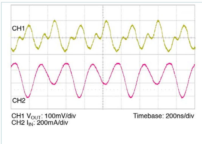
Figure 14 — Output voltage and input current ripple; V_{IN} = 352V , 325W, no C_{OUT}
