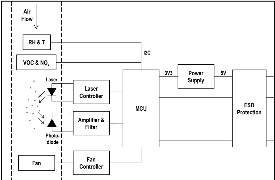
Figure 1 Functional block diagram of the SEN5x. The RH & T and VOC sensors are only contained in the SEN54 and SEN55, the NOx signal is only contained in the SEN55.
