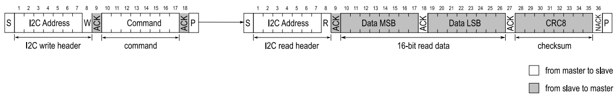
Figure 5. I 2 C transfer types: First a write header is sent to the I 2 C slave, followed by a command, for example "measure T with highest precision". After the measurement is finished the read request directed to this I 2 C slave will be acknowledged and transmission of data will be started by the slave.
