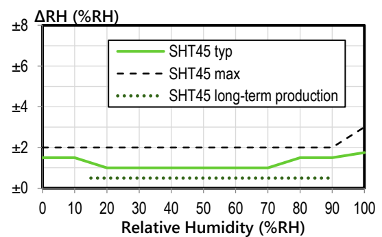
Figure 5. SHT45 typical, maximal and long-term production 11 relative humidity accuracy at 25 °C.
