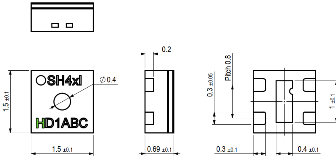
Figure 6. Dimensional drawing of SHT4xI-Analog with filter membrane, including package tolerances (units mm).
