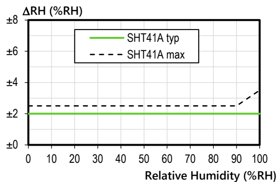
Figure 3. SHT41A typical and maximal relative humidity accuracy at 25 °C.
