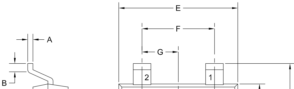
Mechanical Drawing: SOT-23
