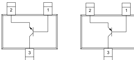
CMST3904 NPN
