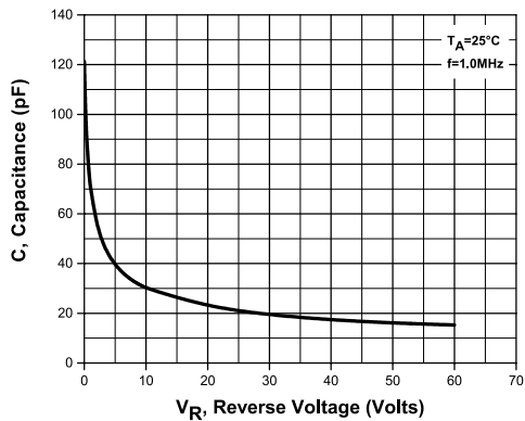
Capacitance for CMSH1-60M
