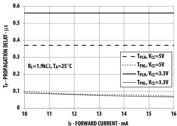
Figure 9 Propagation Delay Time vs Input Current
