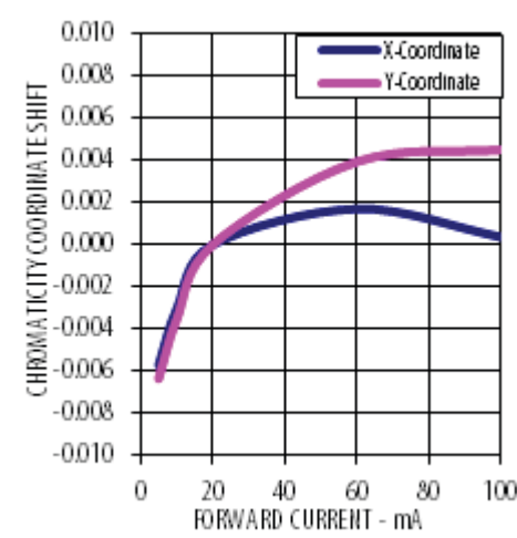
Figure 5 Chromaticity Shift vs. Forward Current
