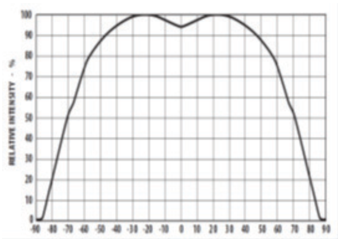
Figure 4 Radiation Pattern
