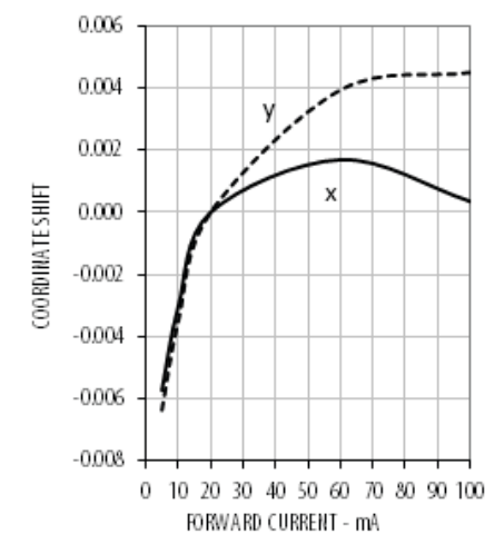
Figure 5 Chromaticity Shift vs. Forward Current
