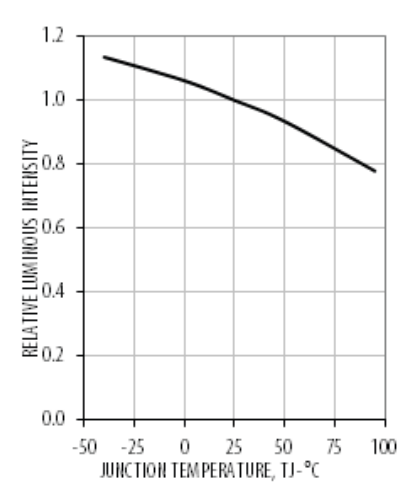
Figure 6 Relative Intensity vs. Temperature
