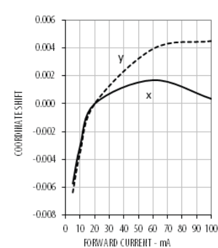
Figure 5 Chromaticity Shift vs. Forward Current
