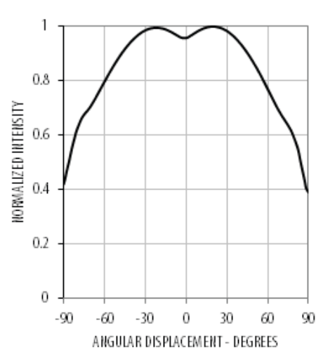
Figure 4 Radiation Pattern
