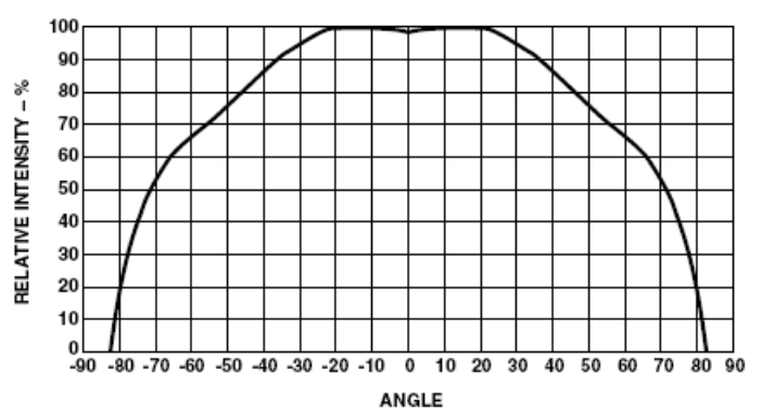
Figure 4 Radiation Pattern
