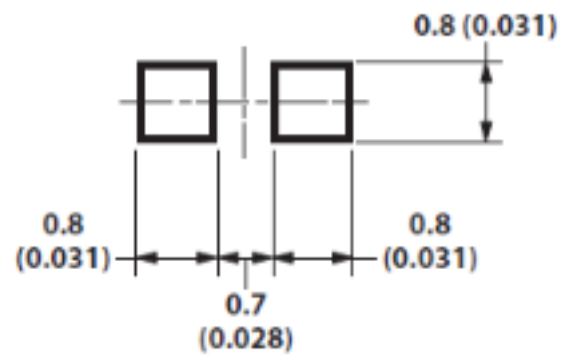
Recommended Solder Pad
