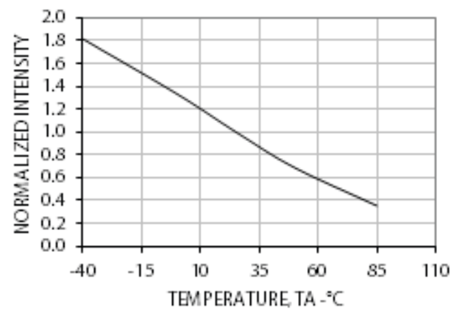
Figure 5 Relative Intensity vs. Temperature
