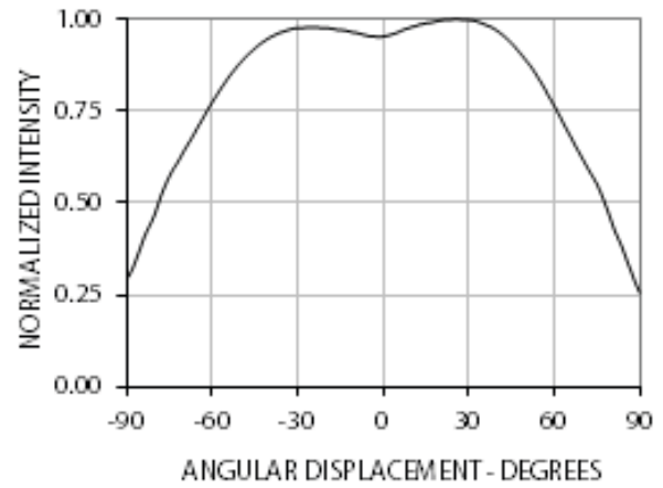
Figure 8 Radiation Pattern
