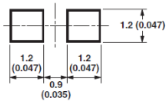
Recommended Solder Pad
