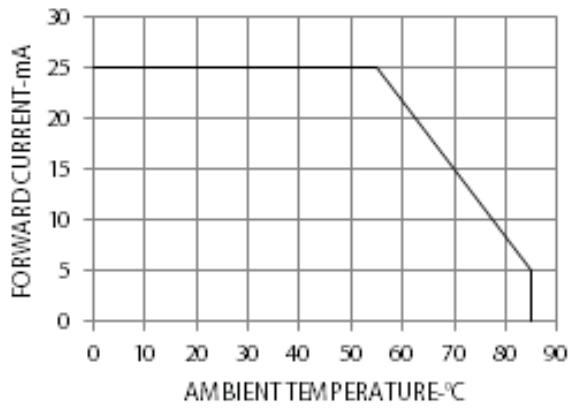
Figure 9 Derating Curve
