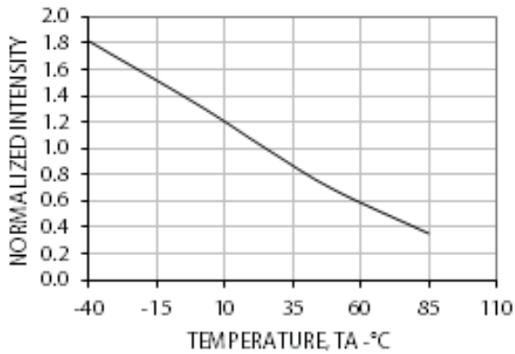
Figure 5 Relative Intensity vs. Temperature
