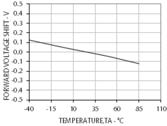
Figure 7 Forward Voltage Shift vs. Temperature
