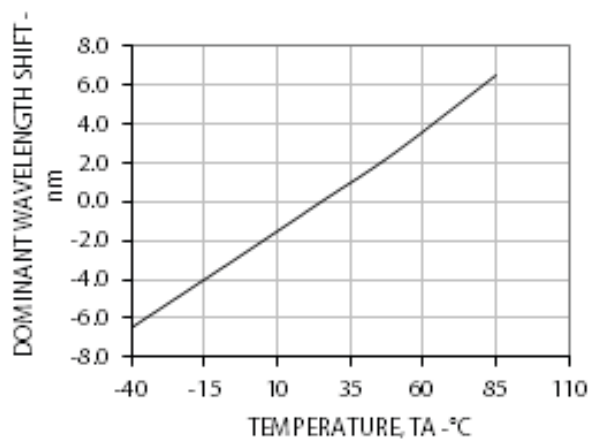
Figure 6 Dominant Wavelength Shift vs. Temperature
