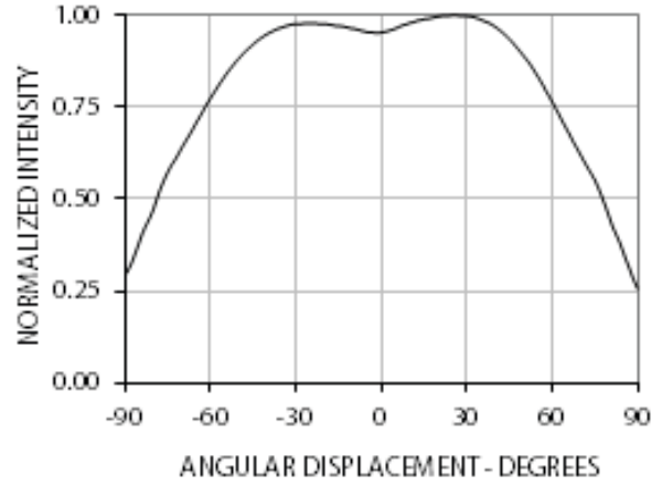
Figure 8 Radiation Pattern
