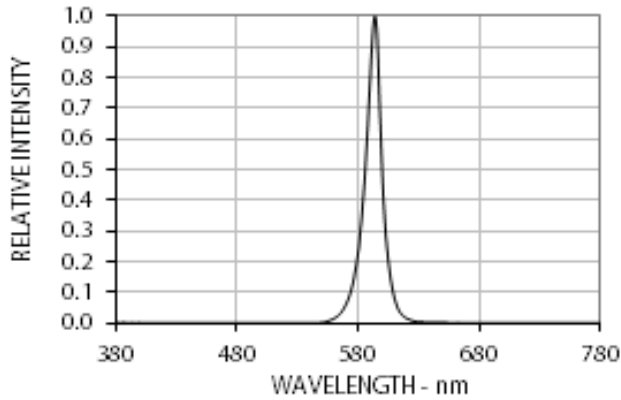
Figure 1 Spectrum
