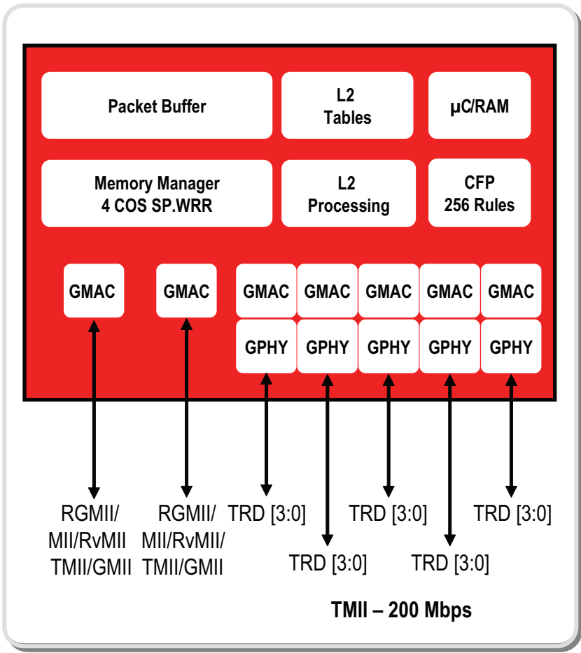
BCM53125 Block Diagram
