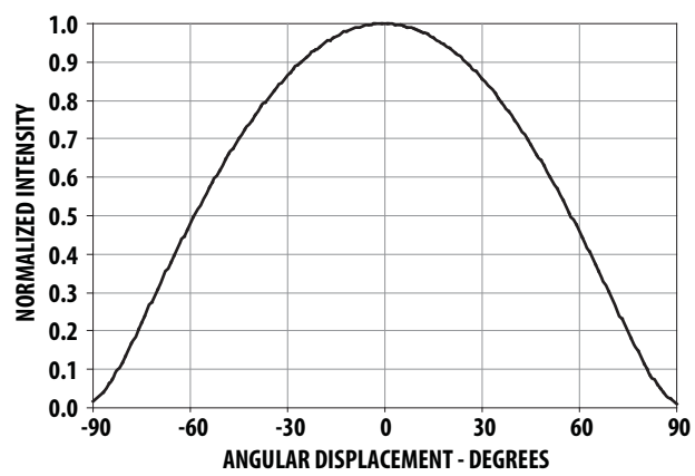
Figure 11. Radiation Pattern
