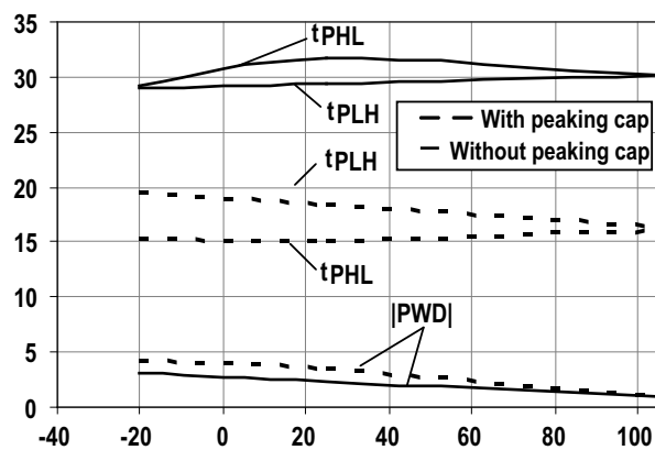
(i) V_{DD} = 5V , C_{peak} = 100 \text{ pF} , R_{limit} = 530\Omega
