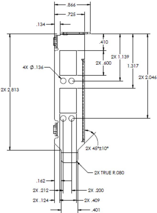
Figure 6: Low-Profile Bracket Outline and Dimensions
