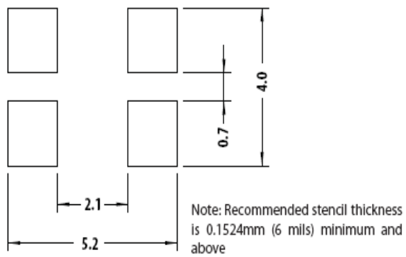
Figure 9: Recommended Soldering Land Pattern
