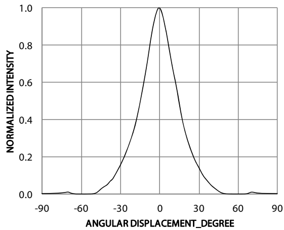
Figure 6a: Radiation Pattern for X axis
