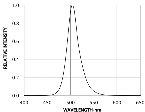
Figure 1: Relative Intensity vs Wavelength
