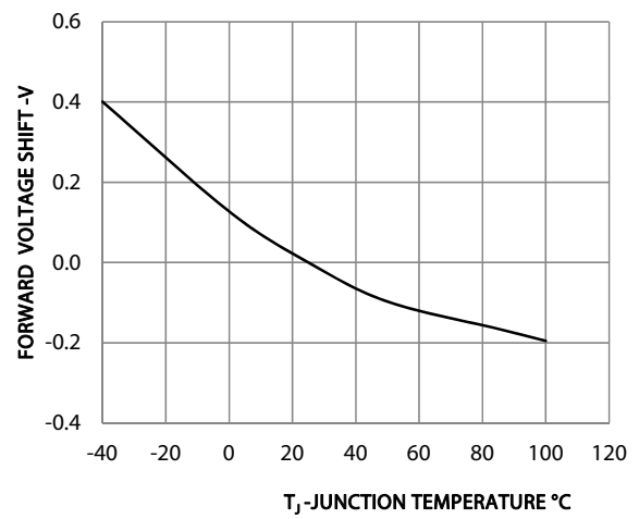
Figure 8: Forward Voltage Shift vs Junction Temperature
