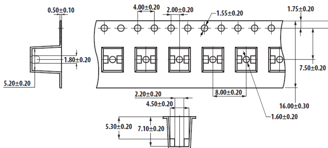
Figure 10 Carrier Tape Dimension
