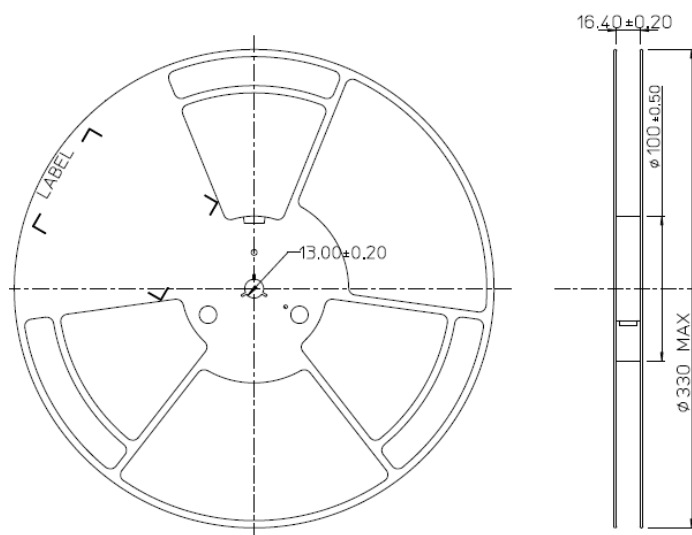
Figure 11 Reel Dimension
