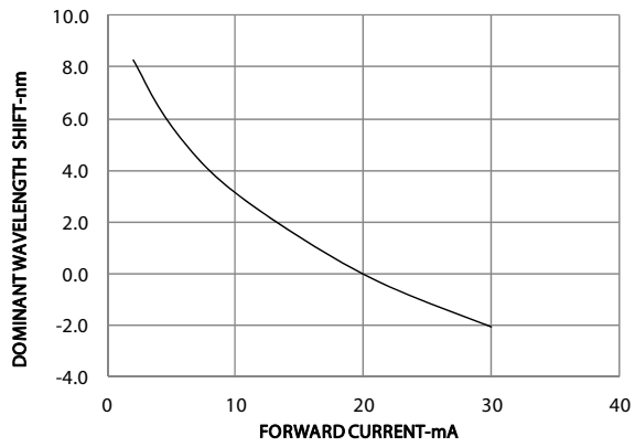
Figure 5: Dominant Wavelength Shift vs Forward Current
