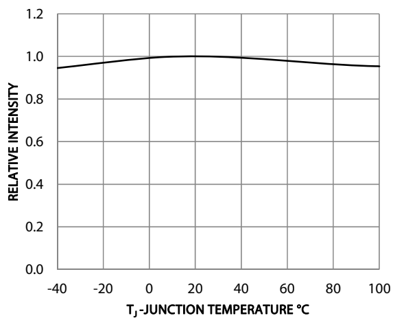
Figure 7: Relative Intensity Shift vs Junction Temperature
