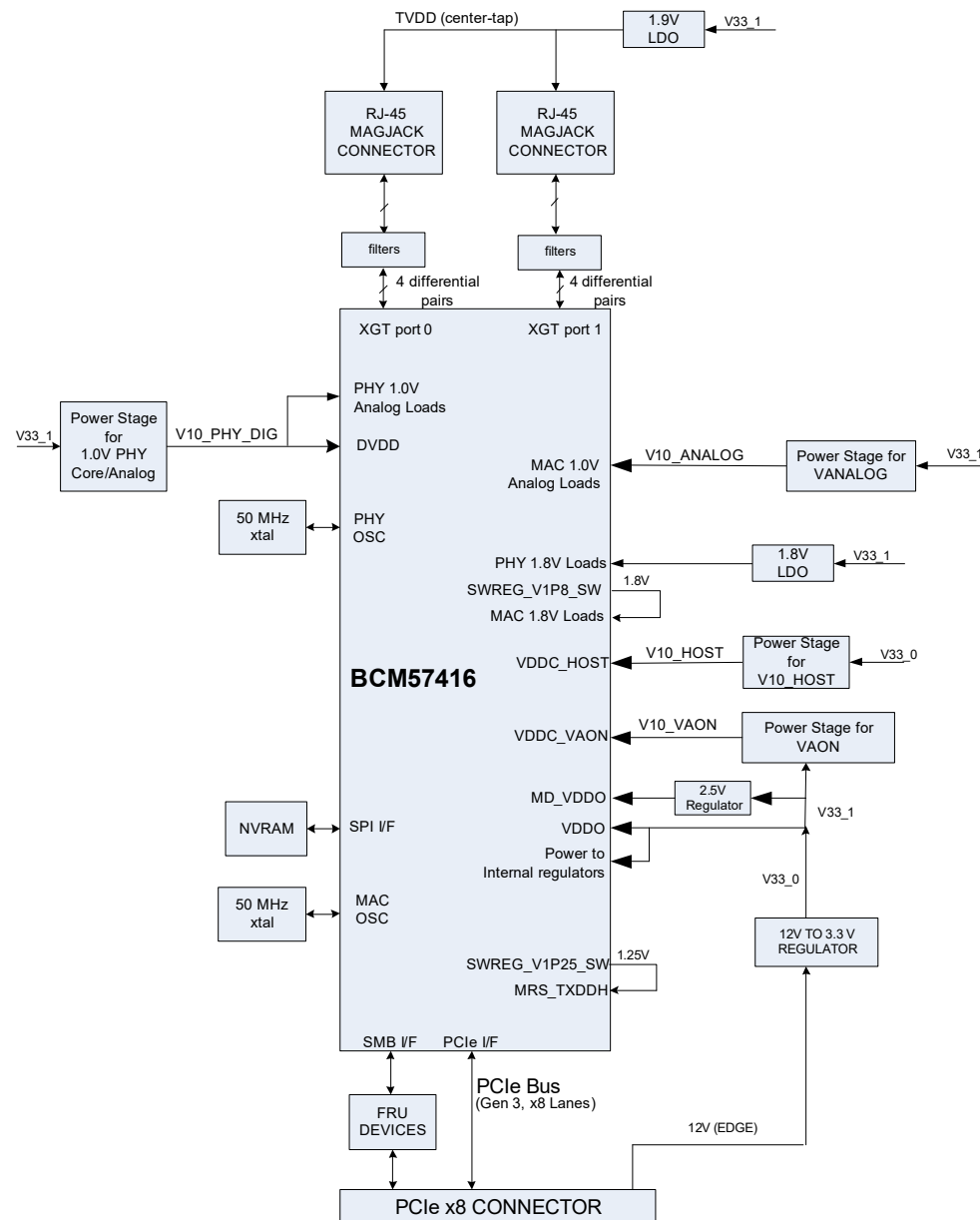
Figure 2: BCM957416A4160C Block Diagram
