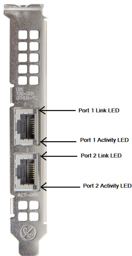
Figure 3: Activity and Link LED Locations
