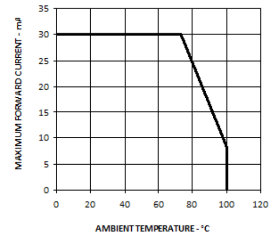
Figure 6: Maximum Forward Current vs. Ambient Temperature. Derated based on T_{jmax} 110° C, R_{thja} 600°C/W.
