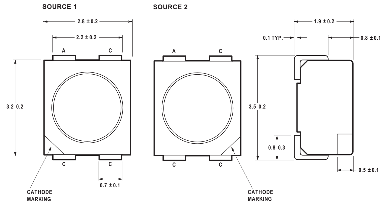
Figure 1: Package Drawing
