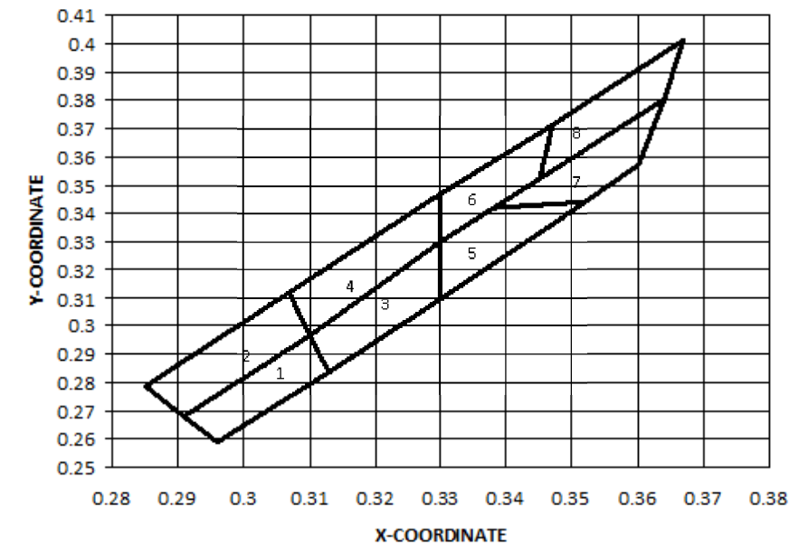
Figure 2: Chromaticity Diagram
