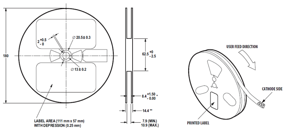
Figure 9: Reel Dimensions
