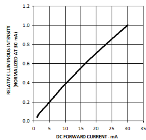
Figure 4: Relative Intensity vs. Mono Pulse Current
