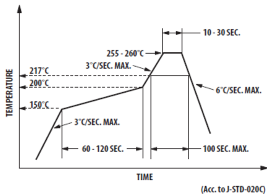
Recommended Pb free reflow solder profile
