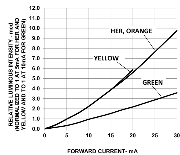
Figure 7: Relative Luminous Intensity vs. Forward Current
