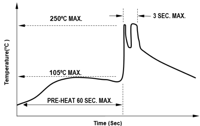
Figure 9: Recommended Wave Soldering Profile
