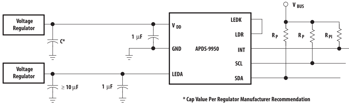
Figure 18a. Circuit Implementation using Separate Power Supplies
