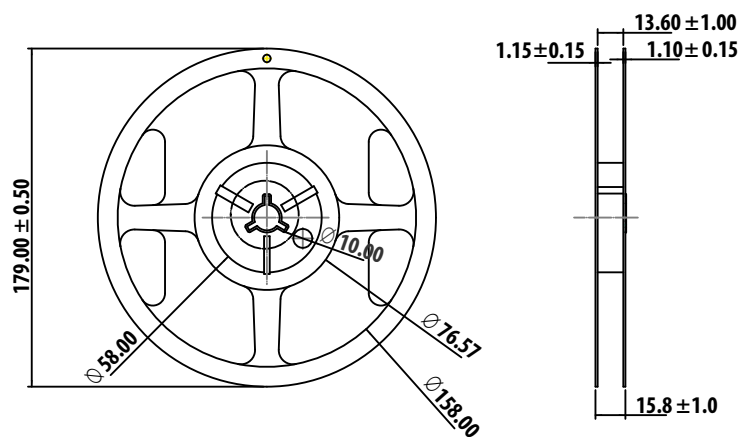
Figure 11. Reel Dimensions
