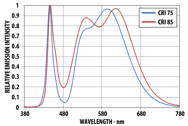
Figure 4. Spectrum Distribution
