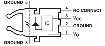
HFBR-2525EZ Receiver, top view
