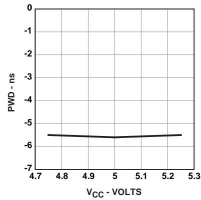
Figure 10. Typical POF receiver pulse width distortion vs. power supply voltage at mid optical power, (-6 dBm,pk, 12 MBd)
