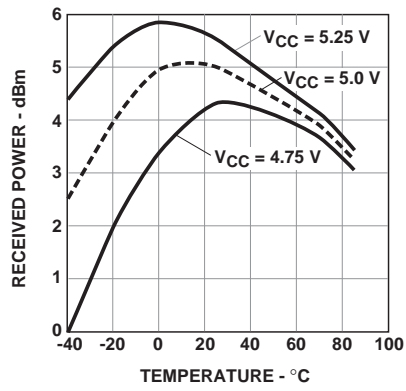
Figure 7. Typical POF receiver overdrive, P_{RL,max} , at 12 MBd, vs. temperature and power supply voltage
