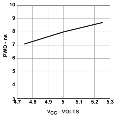
Figure 9. Typical POF receiver pulse width distortion vs. power supply voltage at high optical power (0 dBm,pk, 12 MBd)
