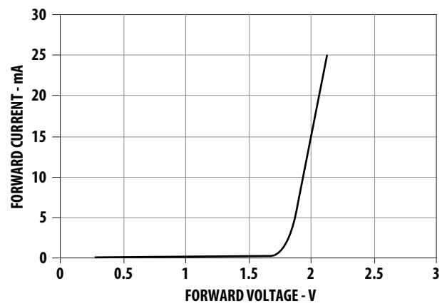
Figure 8. Forward Voltage Vs Current
