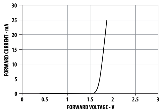
Figure 14. Forward Voltage Vs Current
