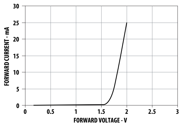
Figure 2. Forward Voltage Vs Current
