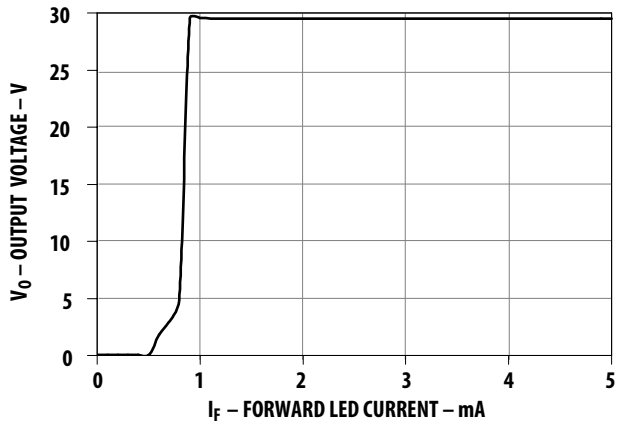
Figure 15. Transfer characteristics.
