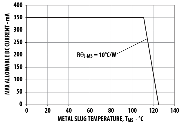
Figure 13. Maximum Forward Current vs. Metal Slug Temperature. Derated based on T_{JMAX} = 125^{\circ}\text{C} , R_{\theta MS} = 10^{\circ}\text{C/W} .
