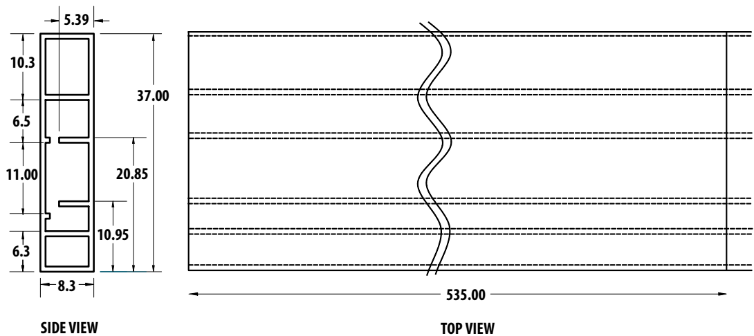
Figure 17. Tube dimensions.
