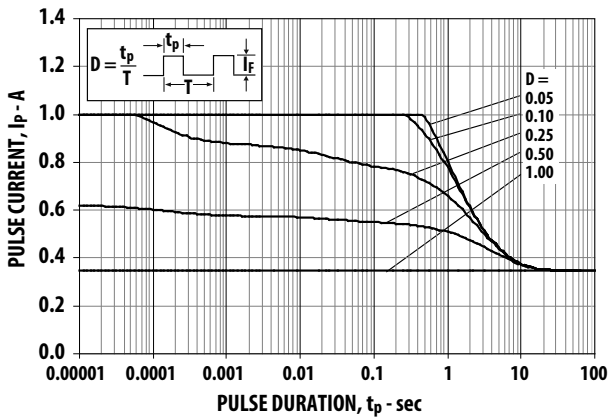
Figure 21 Maximum Pulse Current vs. Pulse Duration. Derated based on T_A = 25^\circ\text{C} , R_{\theta J-A} = 50^\circ\text{C/W} .
