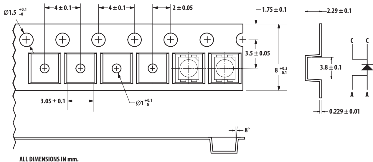
Figure 14. Tape Dimensions
