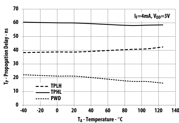
Figure 9. ACFL-6212T (3V) Typical Propagation Delay vs. Temperature
