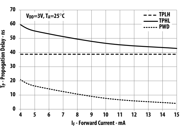
Figure 10. ACFL-6212T (3V) Typical Propagation Delay vs. Input Forward Current
