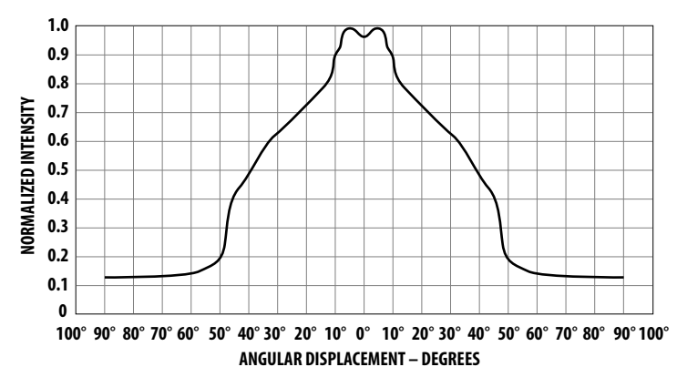
Figure 10: HLMP-P106/-P156
