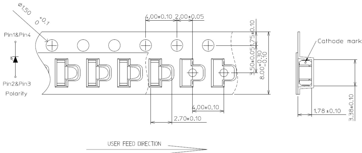
Figure 9: Tape Dimensions (Units: mm)
