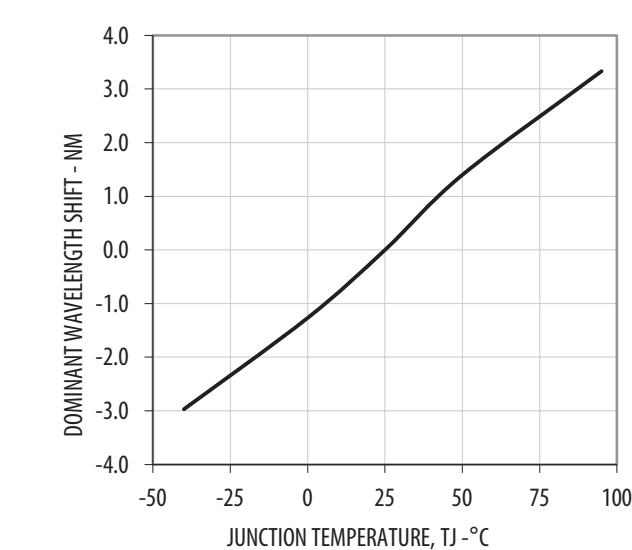
Figure 9: Wavelength Shift vs. Temperature
