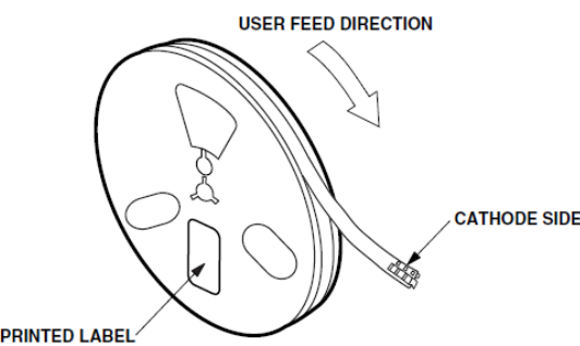
Figure 12: Reel Orientation
