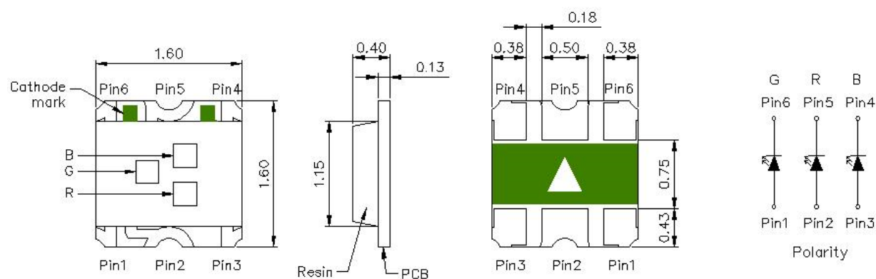
Figure 1: Package Dimensions
