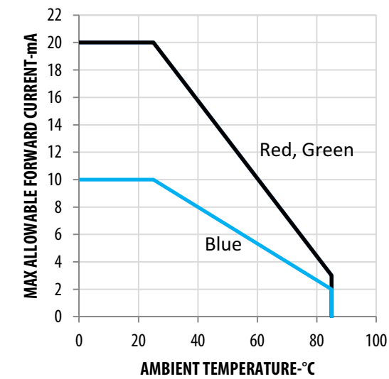
Figure 10: Derating Curve (Single Chip Lit Up)
