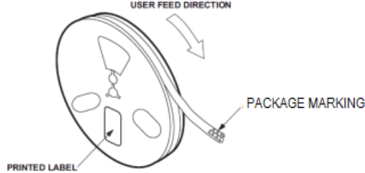
Figure 13: Reel Orientation
