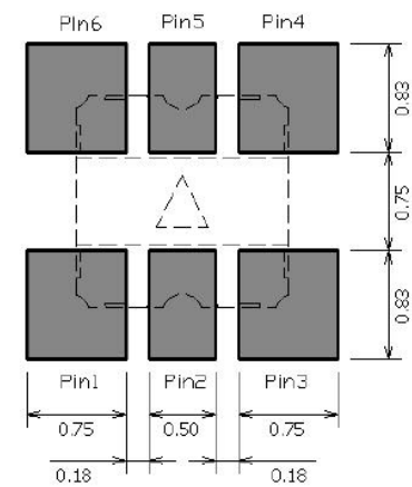
Figure 12: Recommended Solder Pad (Units: mm)
