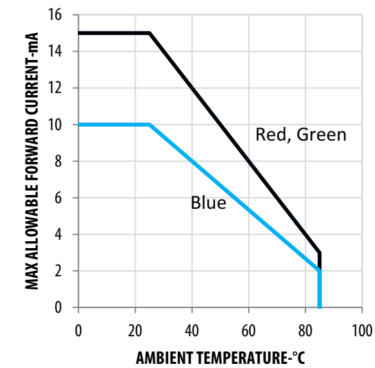
Figure 11: Derating Curve (All Chips Lit Up)
