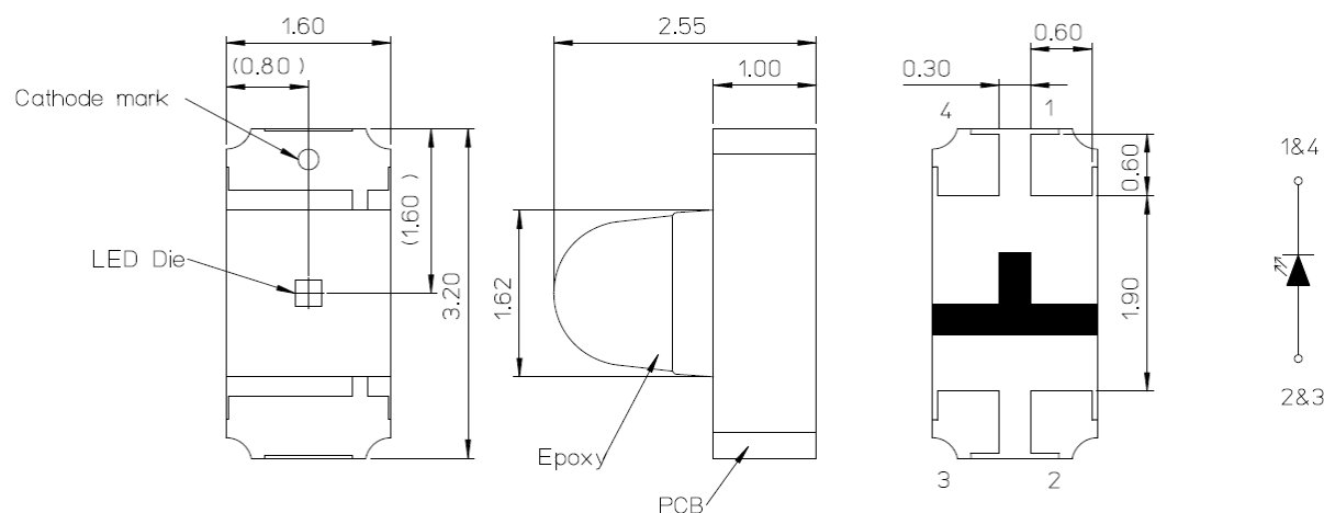
Figure 1: Package Dimensions
