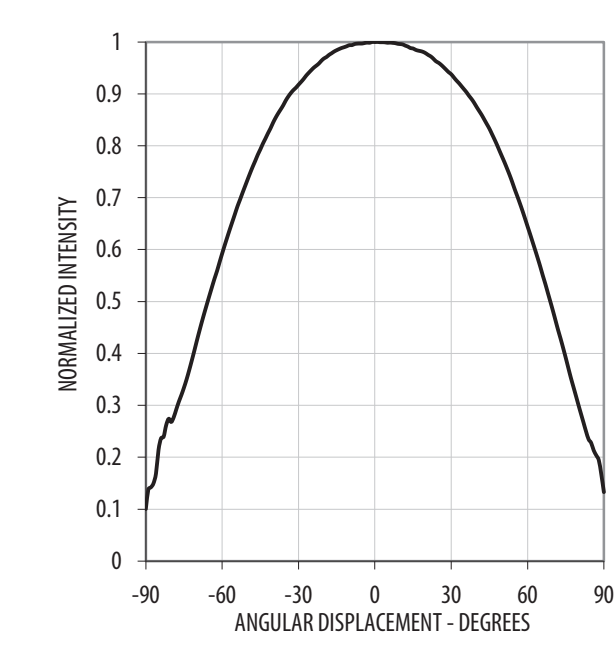
Figure 5: Radiation Pattern
