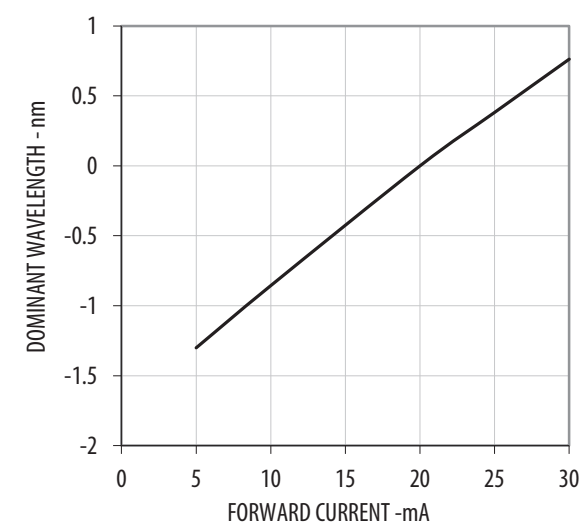
Figure 6: Wavelength Shift vs. Forward Current
