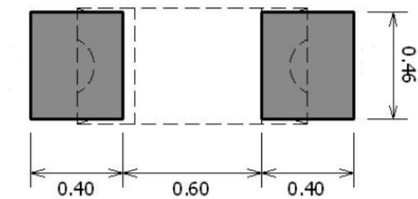
Figure 11: Recommended Solder Pad (Units: mm)
