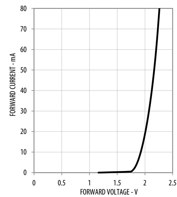
Figure 3: Forward Current vs. Forward Voltage
