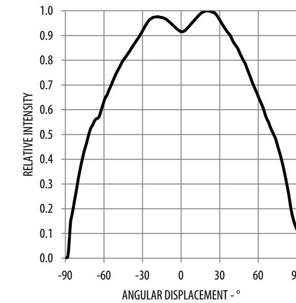
Figure 5: Intensity vs. Angle
