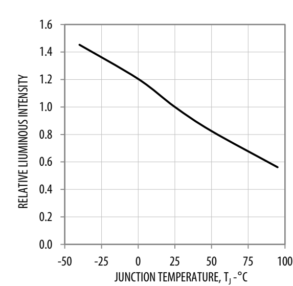
Figure 7: Intensity vs. Temperature
